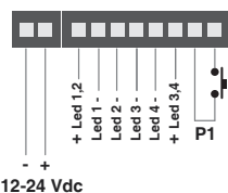
Dimmer mono-colore
